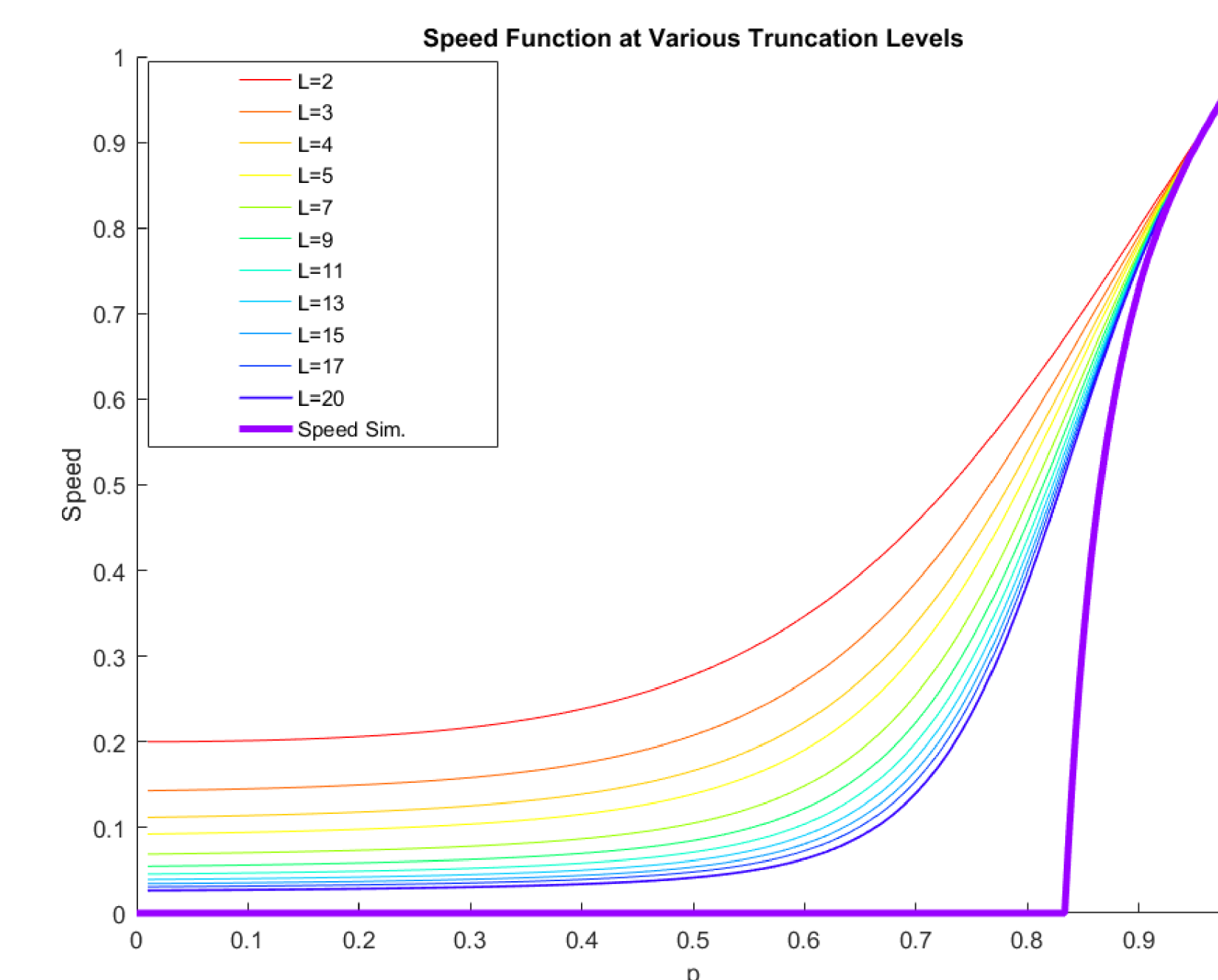
Figure: This graphic shows how the truncated speed approaches the actual speed as L increases with diminishing marginal returns
